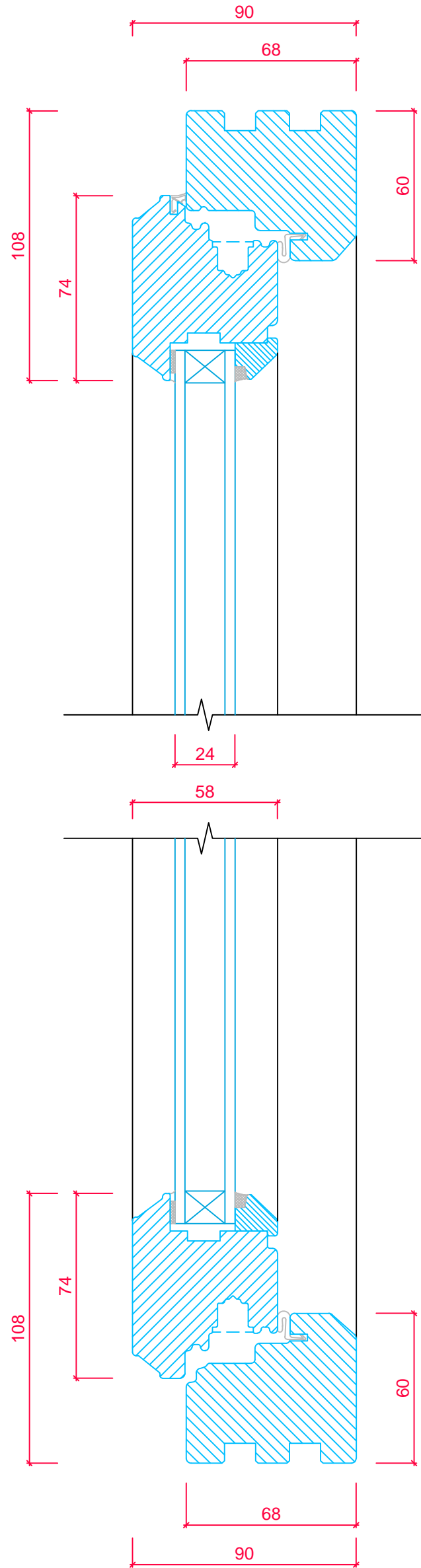
CASEMENT CROSS SECTION 'A-A'
