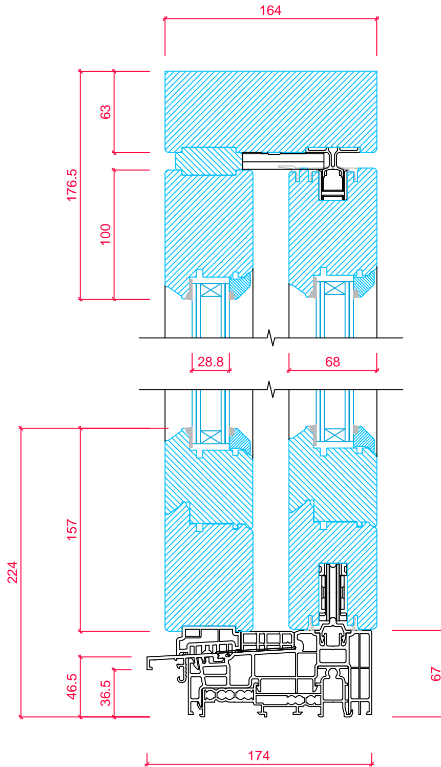
FRAME CROSS SECTION 'A-A'
