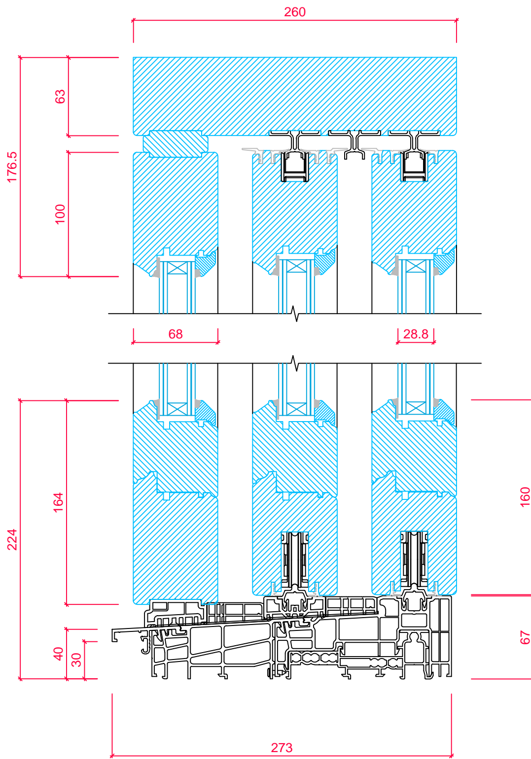
FRAME CROSS SECTION 'A-A'
