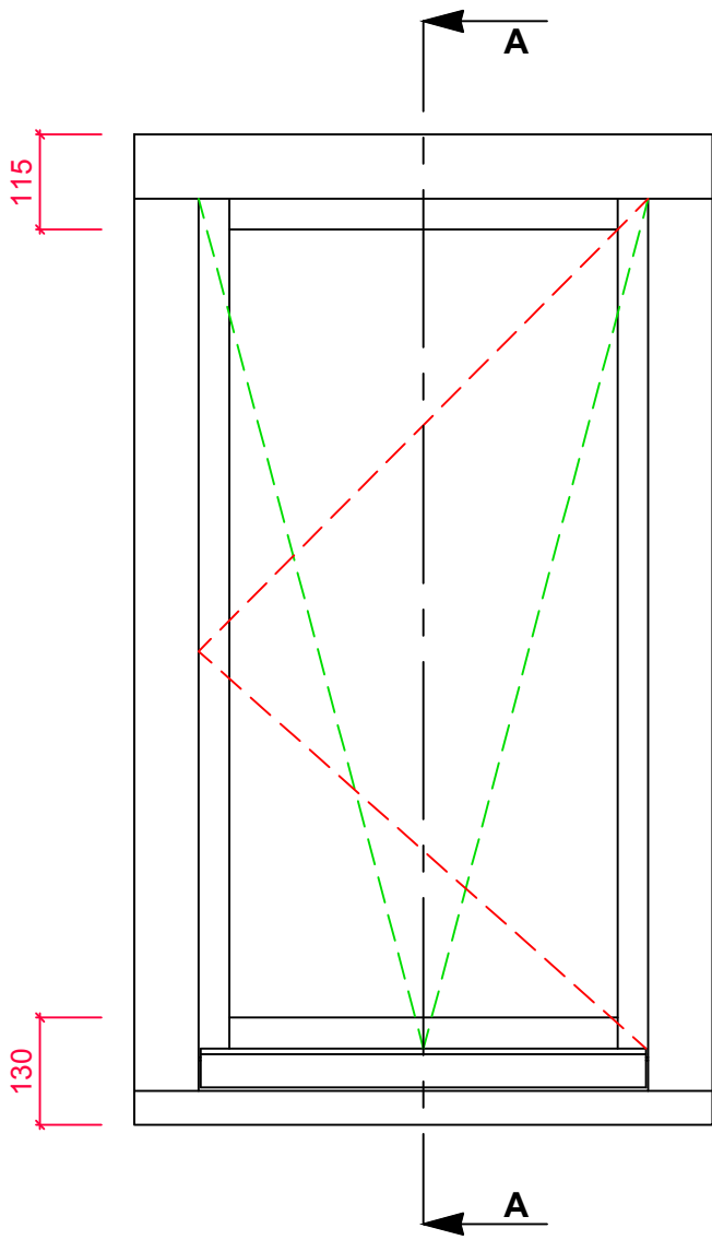
TYPICAL CASEMENT LAYOUT
