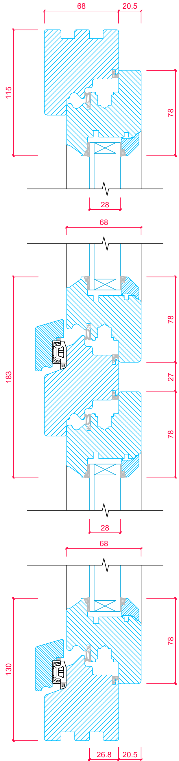
CASEMENT CROSS SECTION 'A-A'
