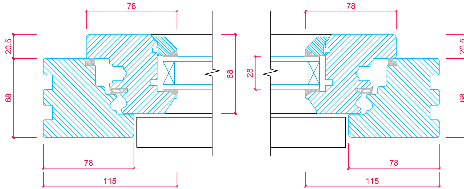
CASEMENT CROSS SECTION 'A-A'
