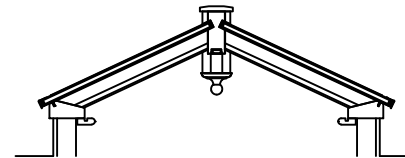
Standard Lantern 8 To Suit Internal Dims Upstand 1660mm x 1115mm
