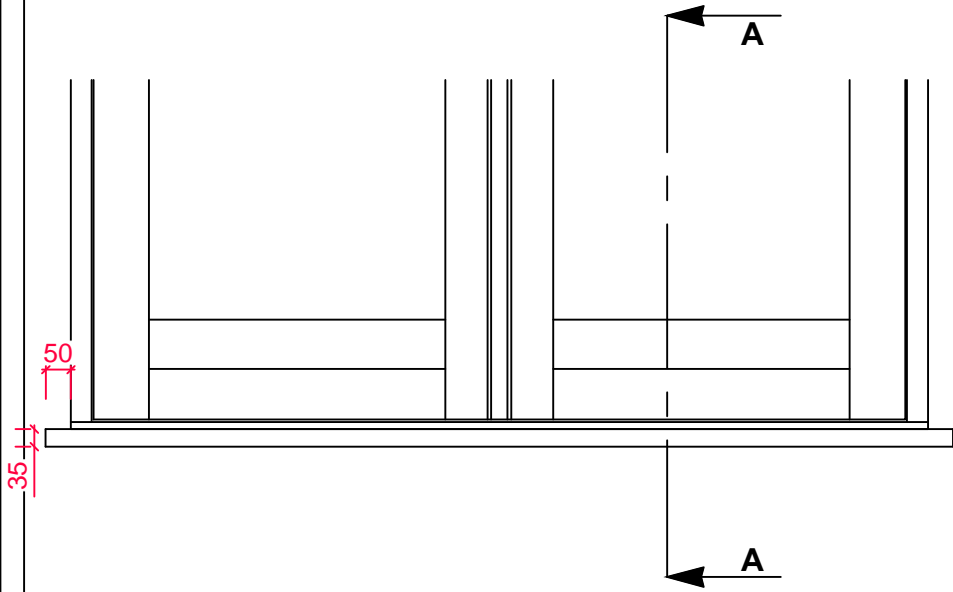
35mm CILL ELEVATION WITH 50mm HORNS L+R
