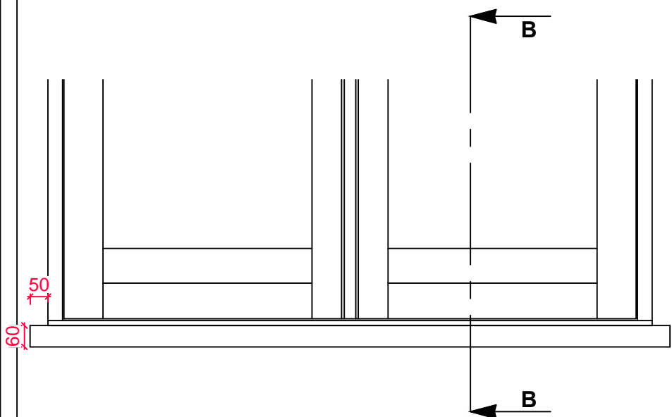
60mm CILL ELEVATION WITH 50mm HORNS L+R
