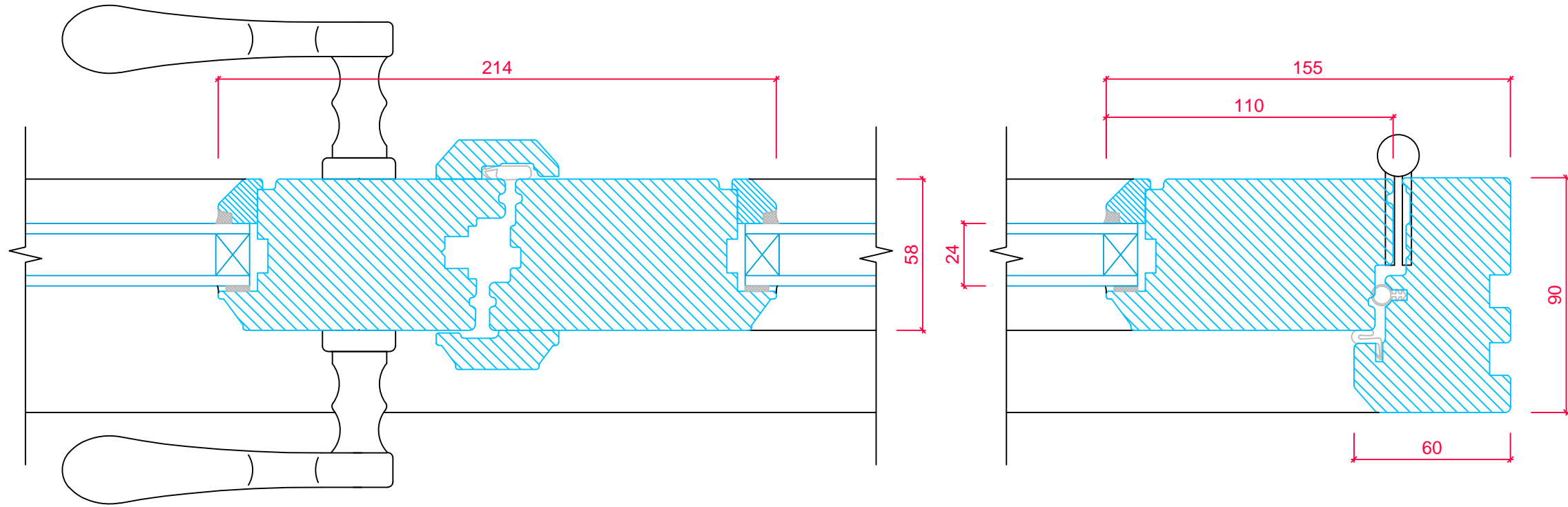
FRAME CROSS SECTION 'A-A'
