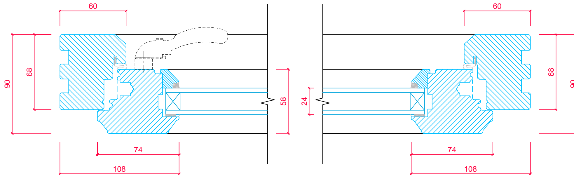
CASEMENT CROSS SECTION 'A-A'
