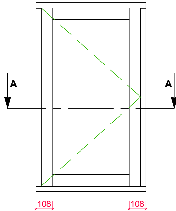
TYPICAL CASEMENT LAYOUT
