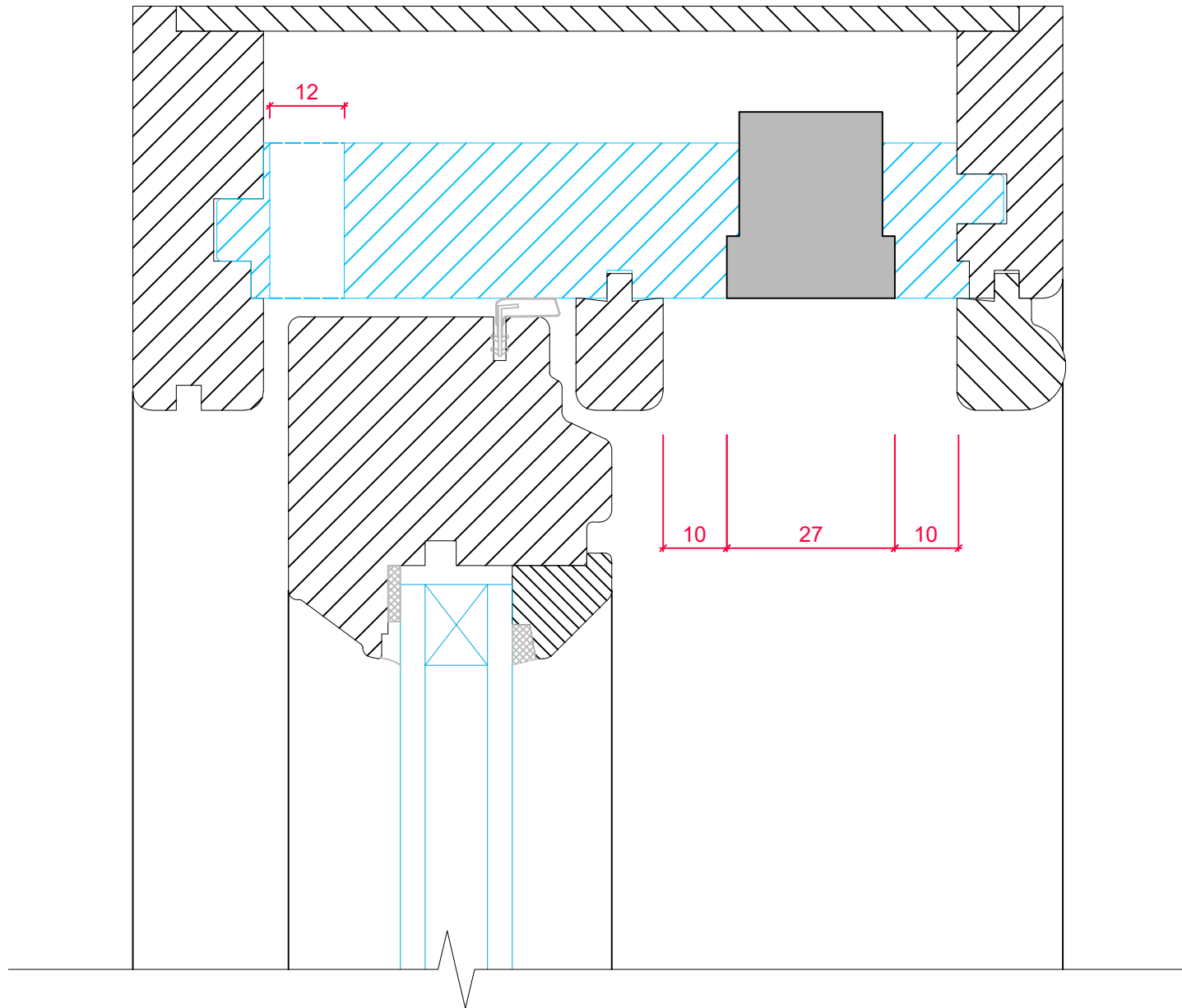
TRICKLE VENT IN HEAD OF FRAME UNAVAILABLE IN SASH TOP RAIL
