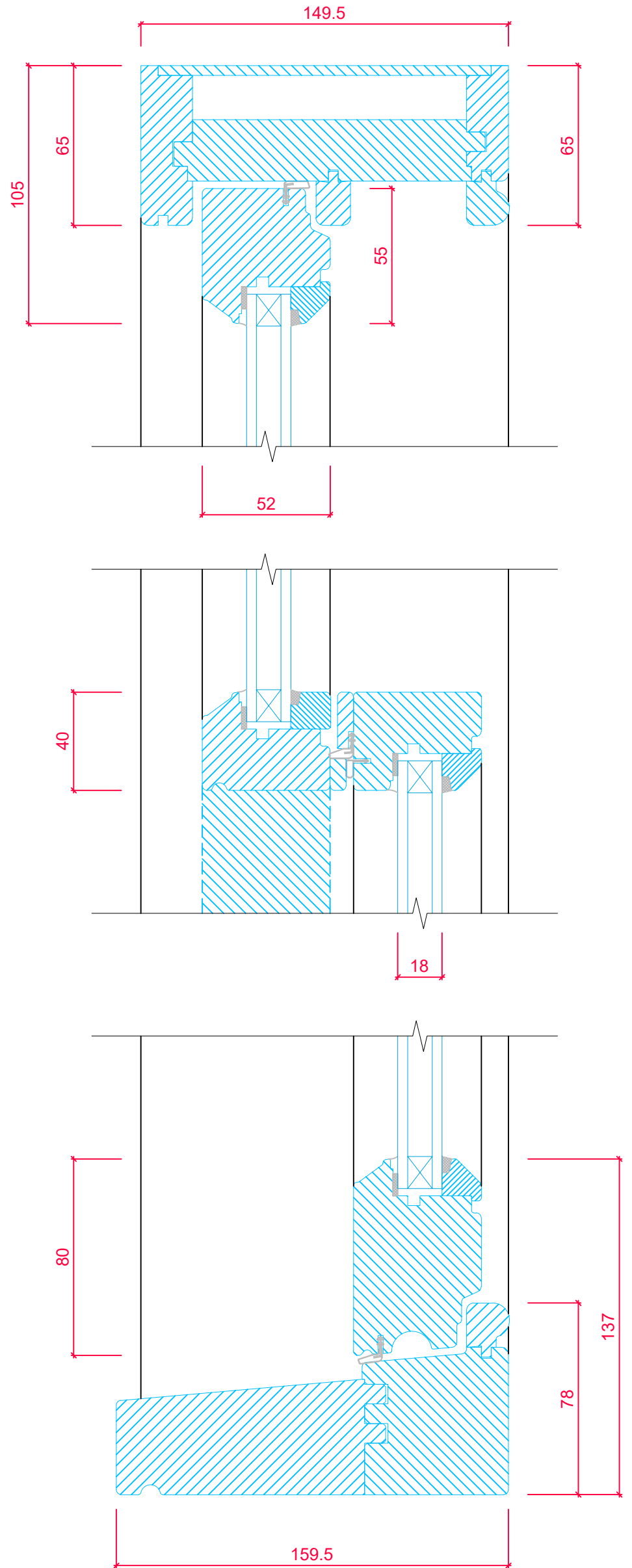
SASH CROSS SECTION 'A-A'
